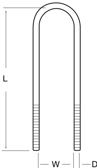
Round Top Style
